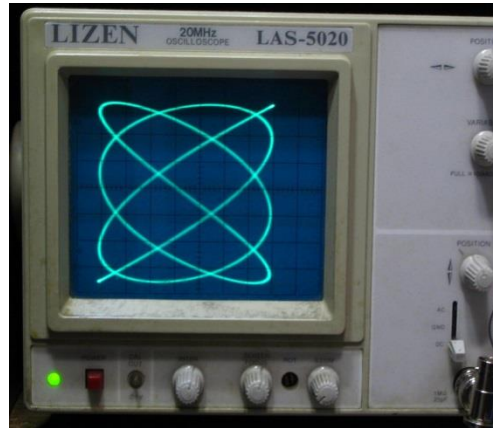
Foto: Wikipedia Lissajous, figure,scope,2,Omegatron
