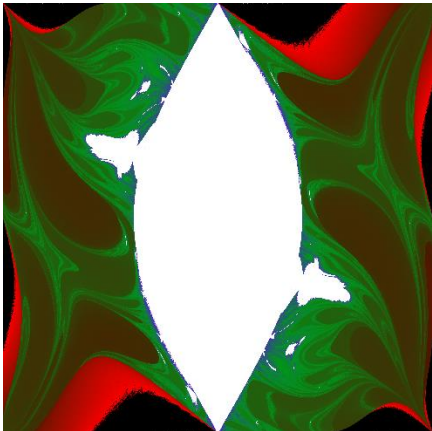
Wikipedia: FurtadoG, Double pendulum, flip time
